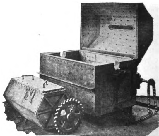
Sherardizing Furnace
